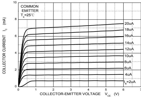
Static Characteristic
