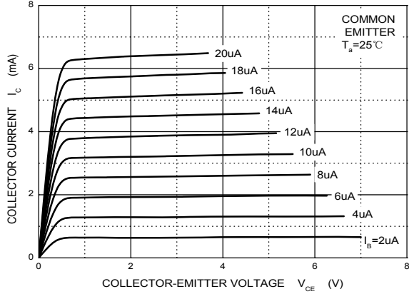
Static Characteristic
